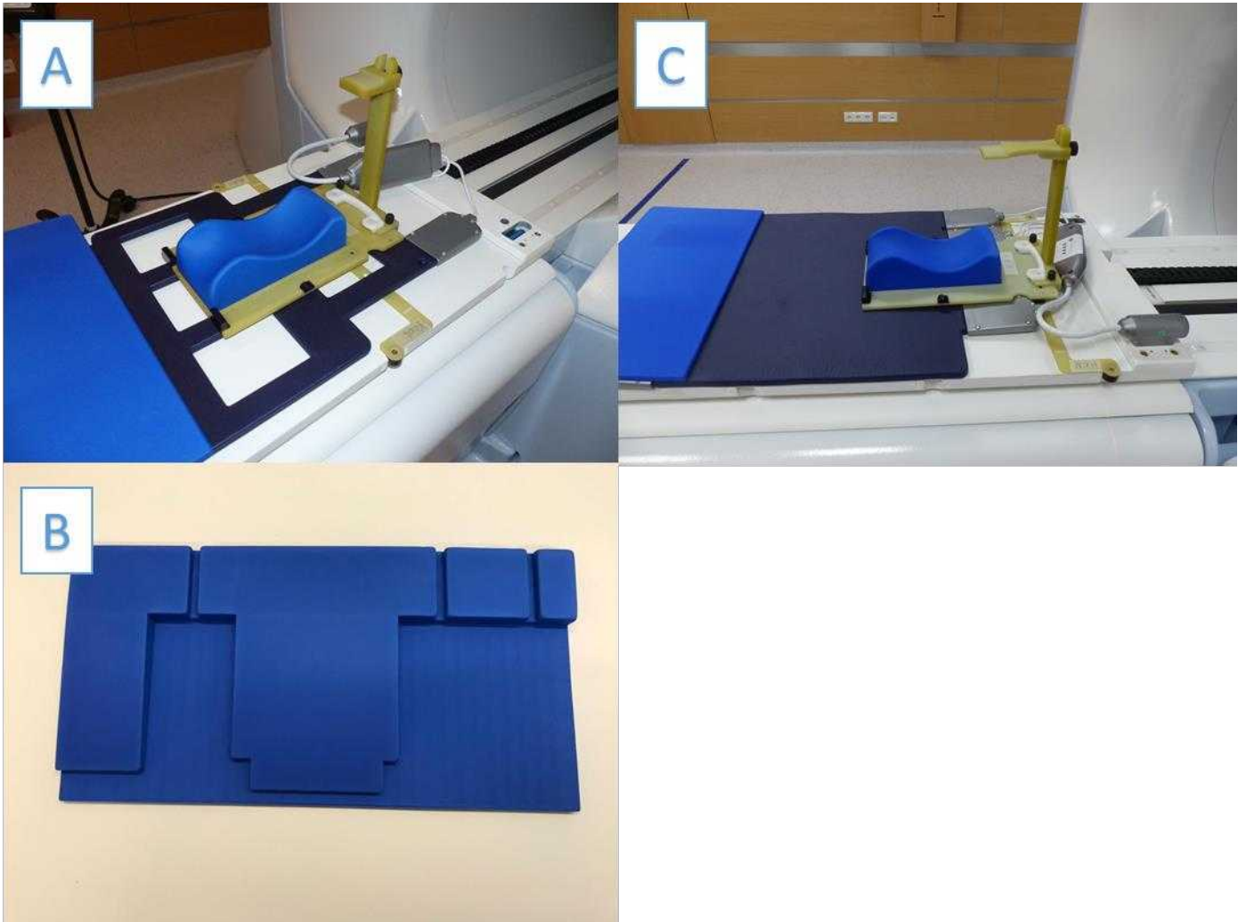
Courtesy of LMU Munich – Viewray MR-Linac. Used devices: HeadSTEP UP VR system for brain (A) or HeadSTEP UP VR H&N system (B) for H&N treatments, HS Flexcoil Holder VR for upper coil positioning, thermoplastic mask, ear plugs, and (C) Flexicoil Comfort Modul VR cushion for flexicoil electronic boxes padding
